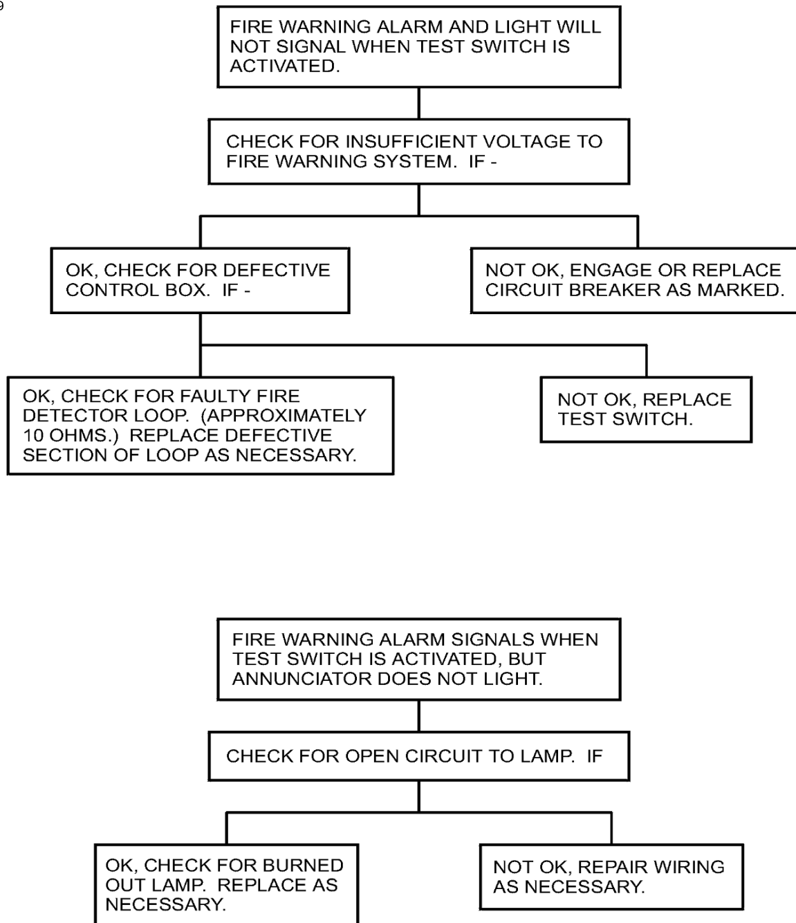
Figure 101 : Sheet 2 : Fire Detection System Troubleshooting Chart
