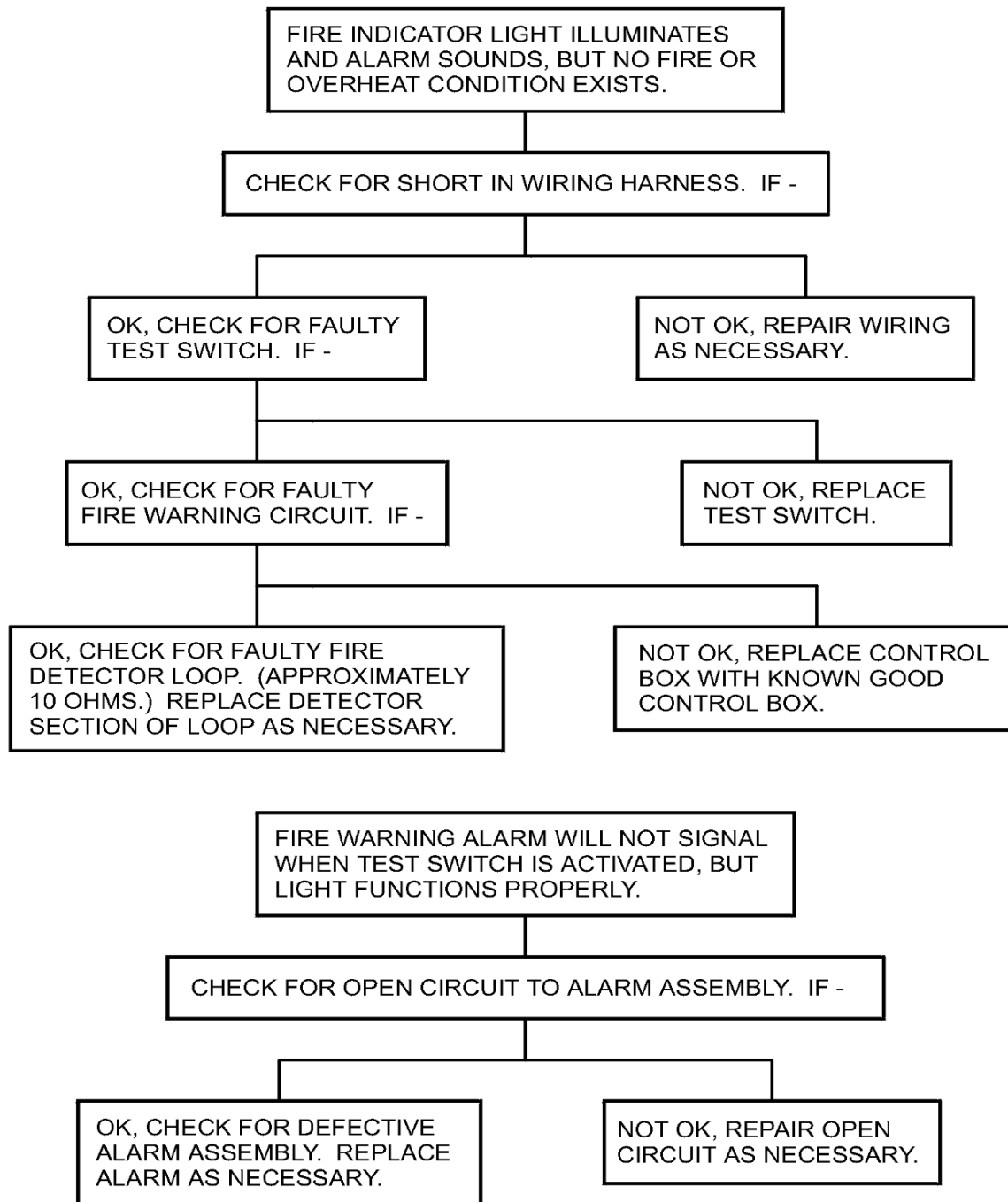
Figure 101 : Sheet 1 : Fire Detection System Troubleshooting Chart
